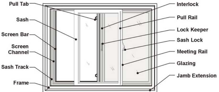
Glider Operator (PVC glider shown)
